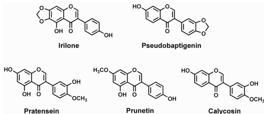
Figure 2. Chemical structures of further isoflavones present in red clover. The aglycon moiety is shown.
