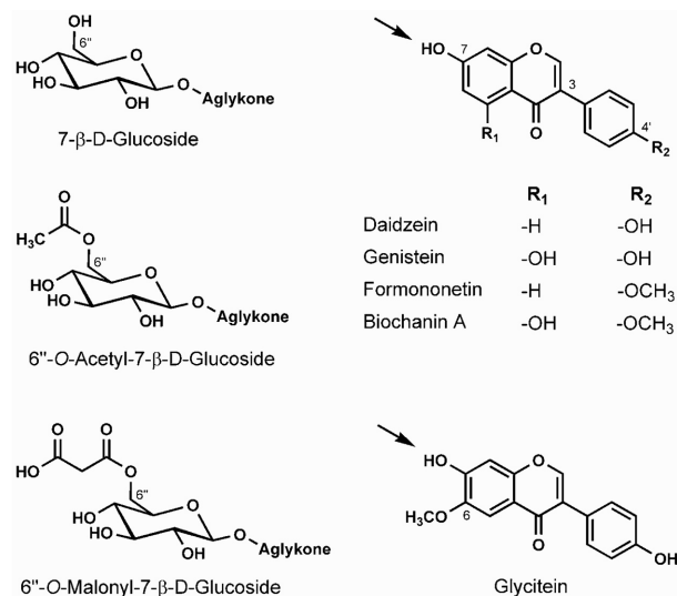
Figure 1. Chemical structures of isoflavones in soy and red clover and their sugar conjugates. The 7-O- \beta -D-glucosides of daidzein, genistein and glycitein are known as daidzin, genistin and glycitin. The arrow in the Figure shows the position of sugar conjugation.
